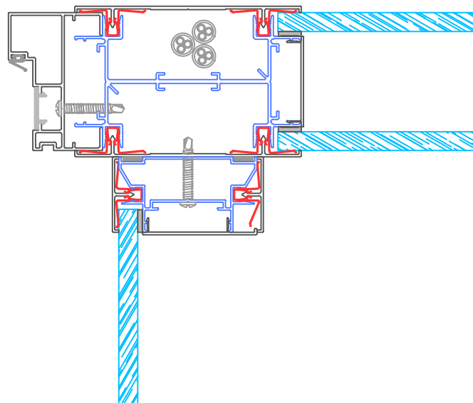
Angle 3 directions
