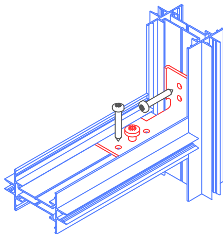
Poteau / Traverse
