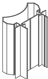
Poteau angle variable ref: EVO300
